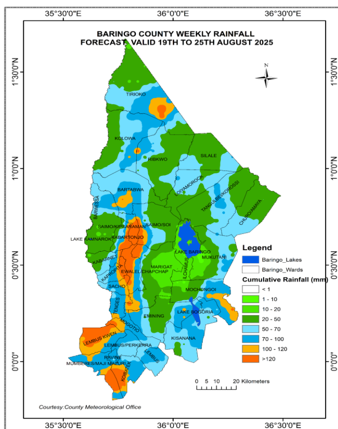
Fig 1. Forecasted cumulative rainfall amounts (mm)
