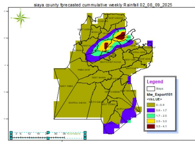
Figure 2: Forecasted cumulative weekly rainfall from 2 nd to 8 th August 2025
