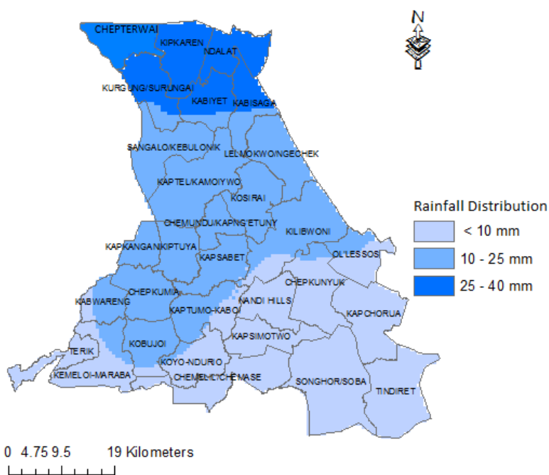
Figure 1: Forecasted Seven-Day total rainfall valid 9 th to 15 th Sept 2025
