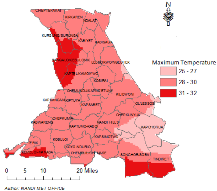
FORECASTED AVERAGE MAXIMUM TEMP FOR 9TH TO 15TH SEP 2025
