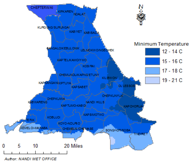
FORECASTED AVERAGE MINIMUM TEMP FOR 9TH TO 15TH SEP 2025
