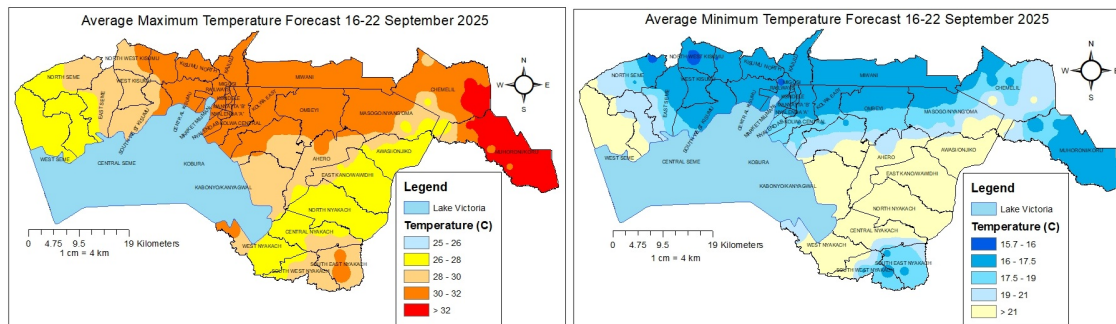
Figure 2: Average maximum (left) and minimum (right) temperature forecasts
