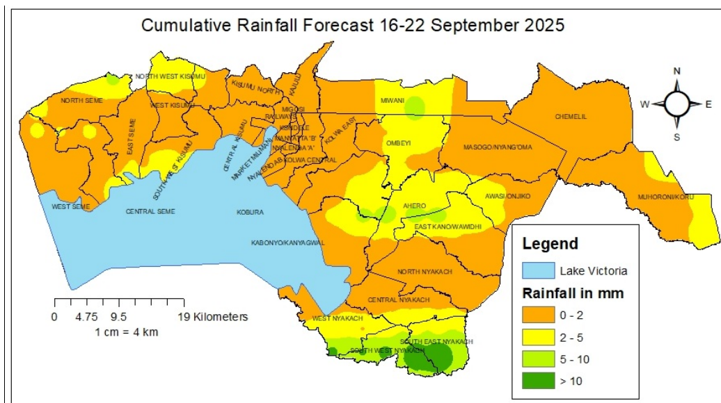
Figure 1: Cumulative rainfall forecast over Kisumu County
