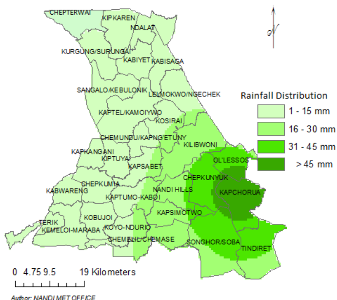
Figure 1: Forecasted Seven-Day total rainfall valid 16 th to 22 nd Sept 2025
