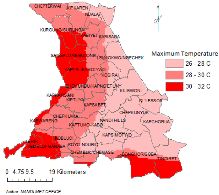
Figure 2: Average Max Temperatures for 16 th – 22 nd Sep 2025
