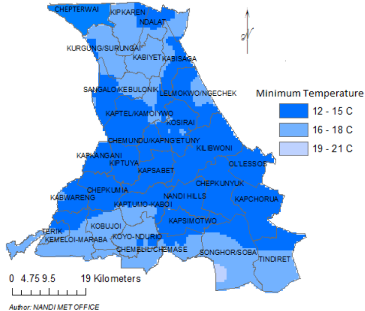
Figure 3: Average Min Temperatures for 16 th – 22 nd Sep 2025
