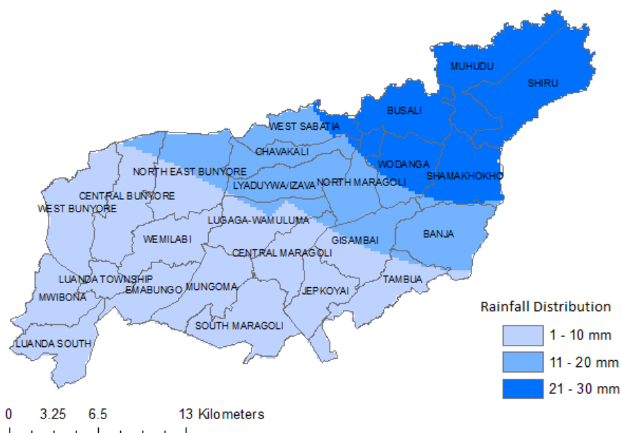
Figure 1: Forecasted Seven-Day total rainfall valid 23 rd to 29 th Sept 2025
