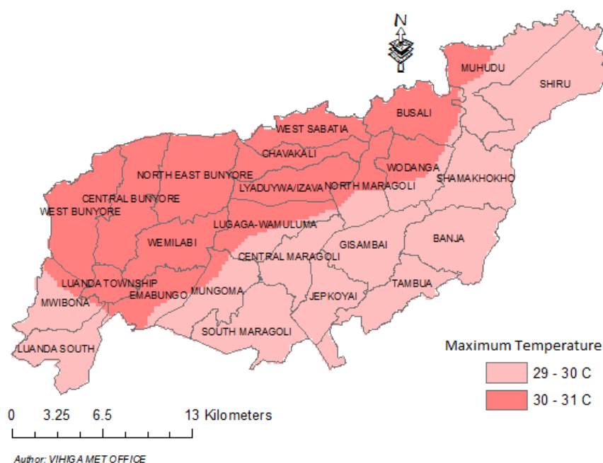
Figure 2: Average Max Temperatures for 23 rd – 29 th Sept 2025
