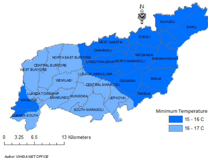
Figure 3: Average Min Temperatures for 23 rd – 29 th Sept 2025
