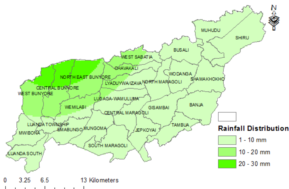
Figure 1: Forecasted Seven-Day total rainfall valid 14 th to 20 th Oct 2025
