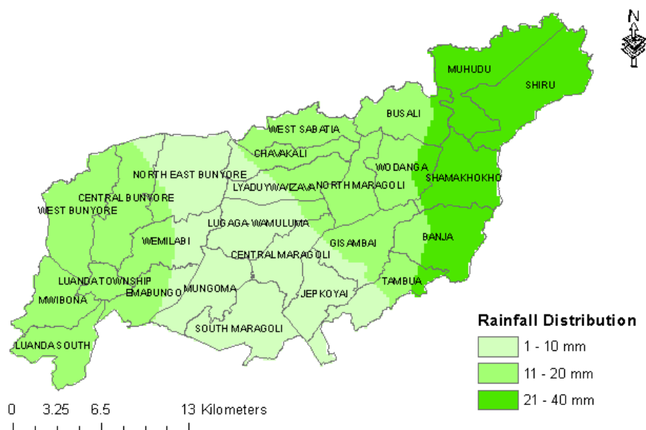
Figure 1: Forecasted Seven-Day total rainfall valid 21 st to 27 th Oct 2025
