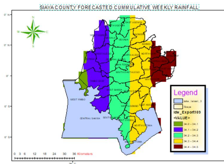
Figure 2: Forecasted cumulative weekly rainfall from 21 st October to 27 th October 2025
