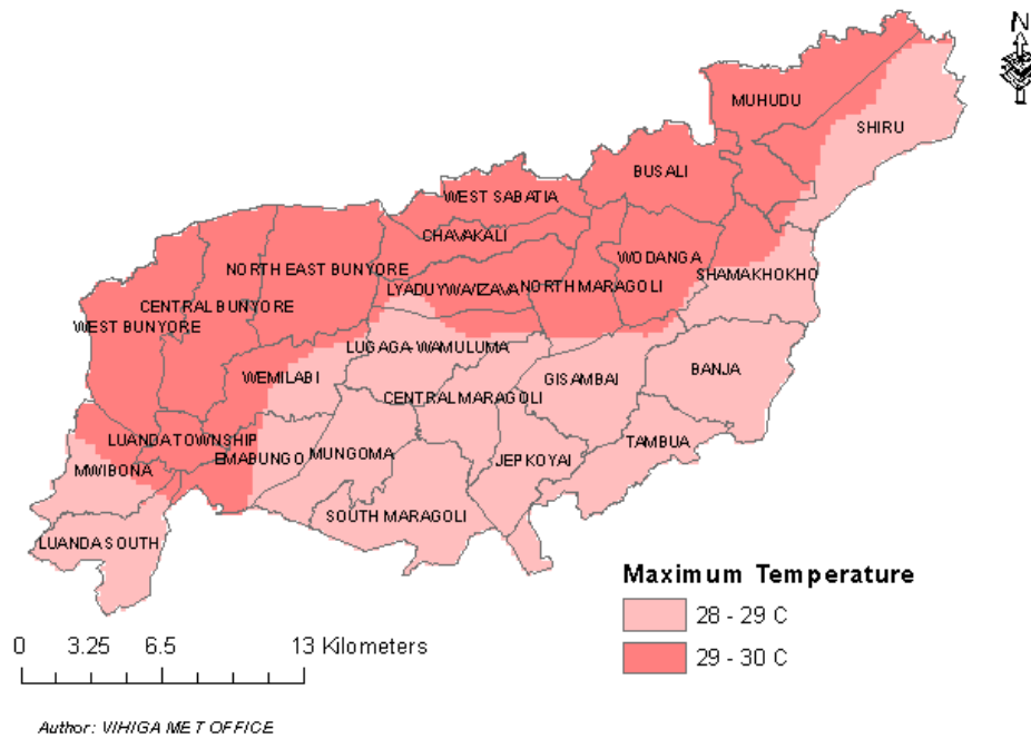
Figure 2: Average Max Temperatures for 4 th to 10 th Nov 2025
