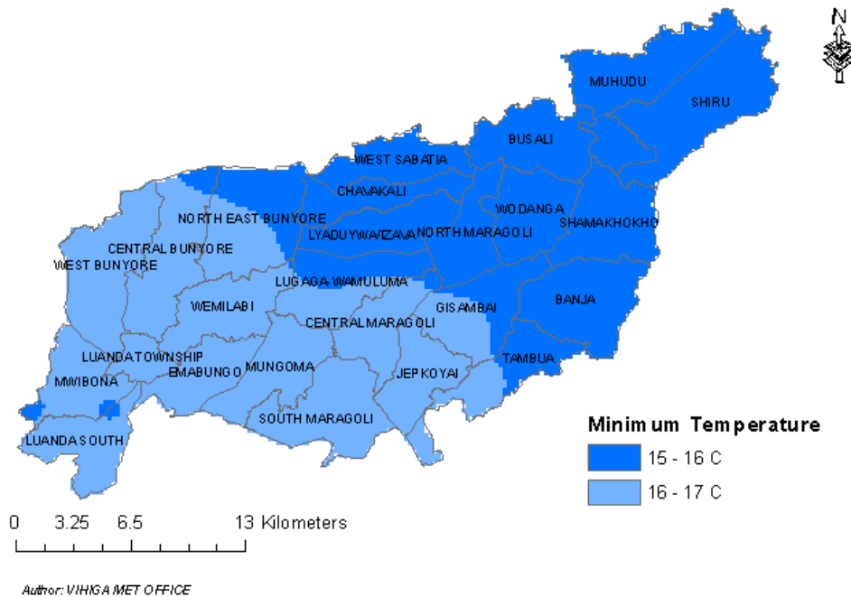
Figure 3: Average Min Temperatures for 4 th to 10 th Nov 2025
