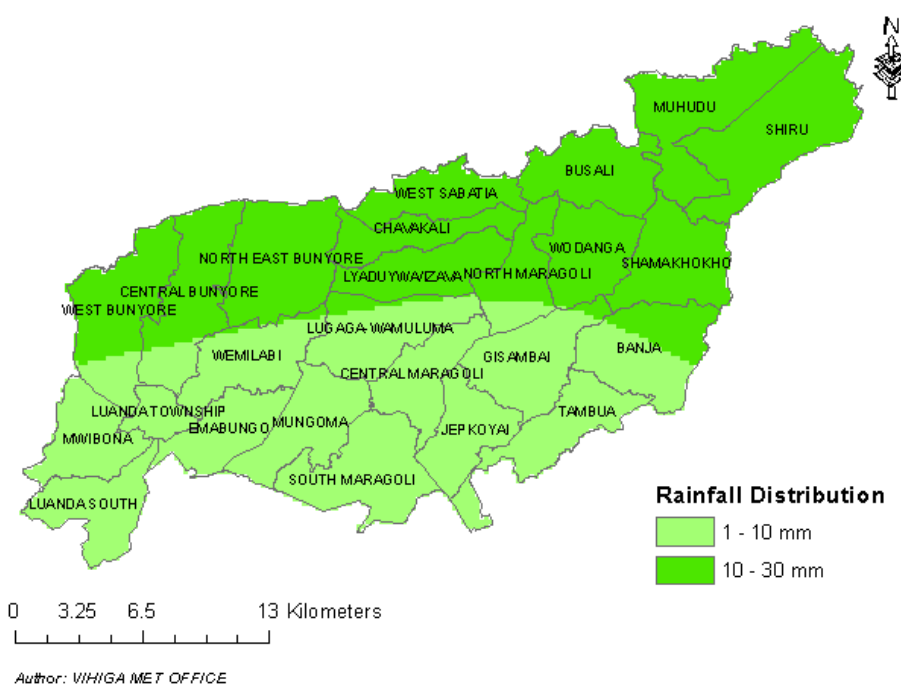
Figure 1: Forecasted Seven-Day total rainfall valid 4 th to 10 th Nov 2025
