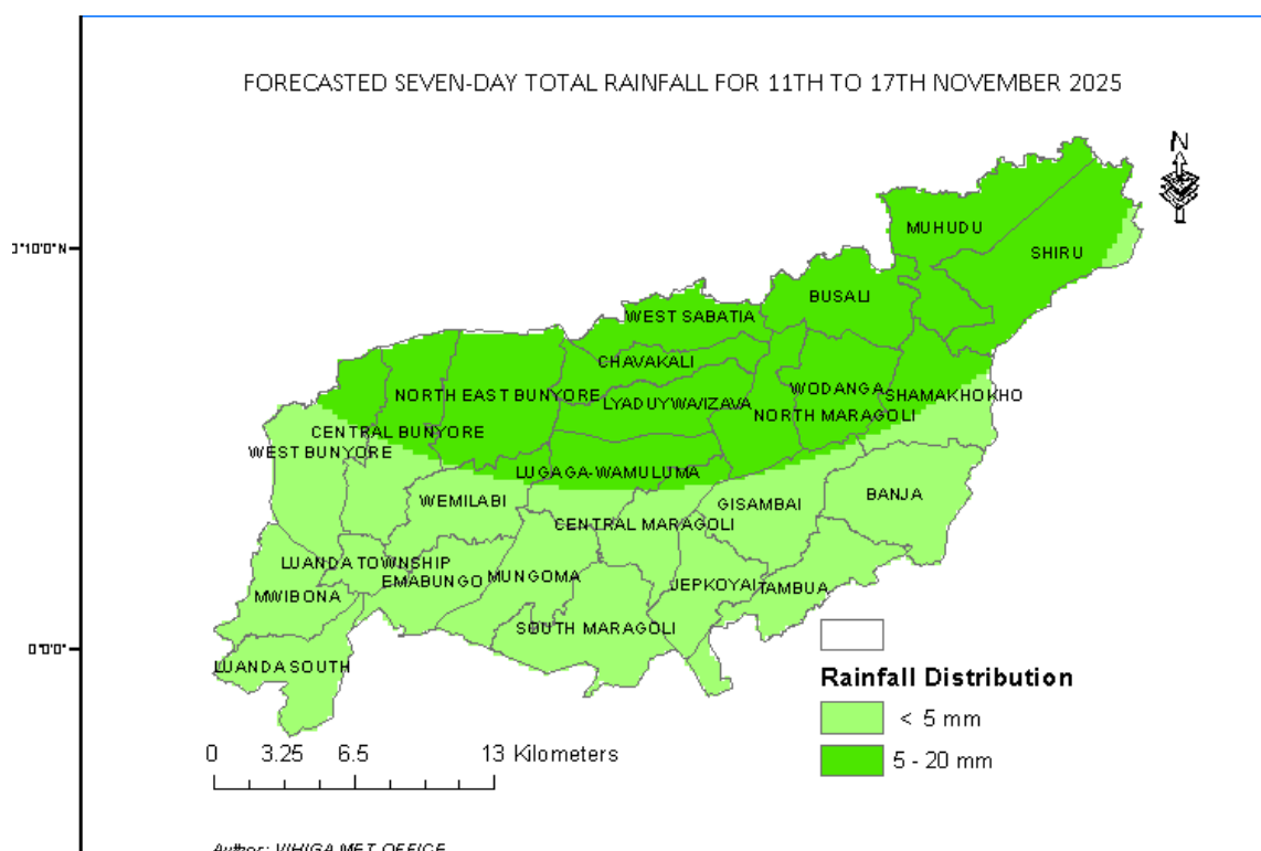
Figure 1: Forecasted Seven-Day total rainfall valid 11 th to 17 th Nov 2025
