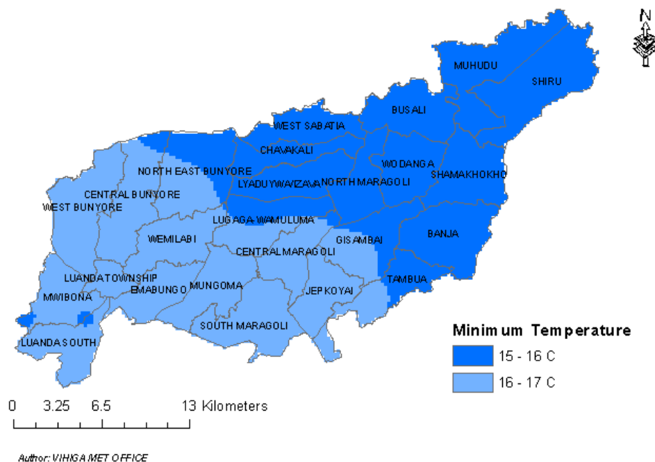
Figure 3: Average Min Temperatures for 11 th to 17 th Nov 2025
