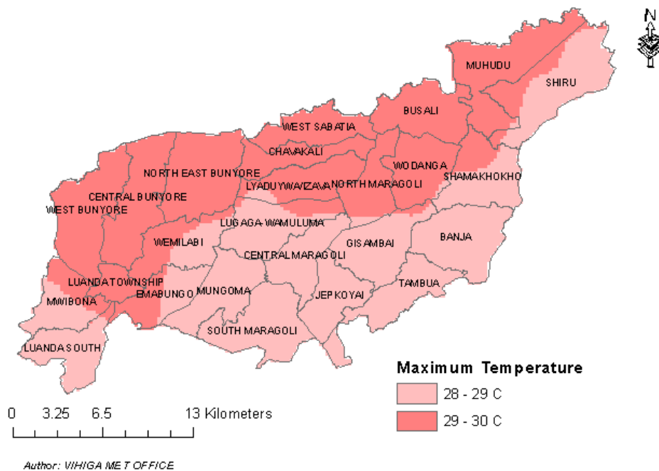
Figure 2: Average Max Temperatures for 11 th to 17 th Nov 2025
