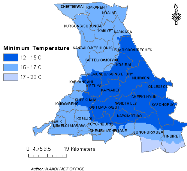
Figure 3: Average Min Temperatures for 18 th to 24 th Nov 2025
