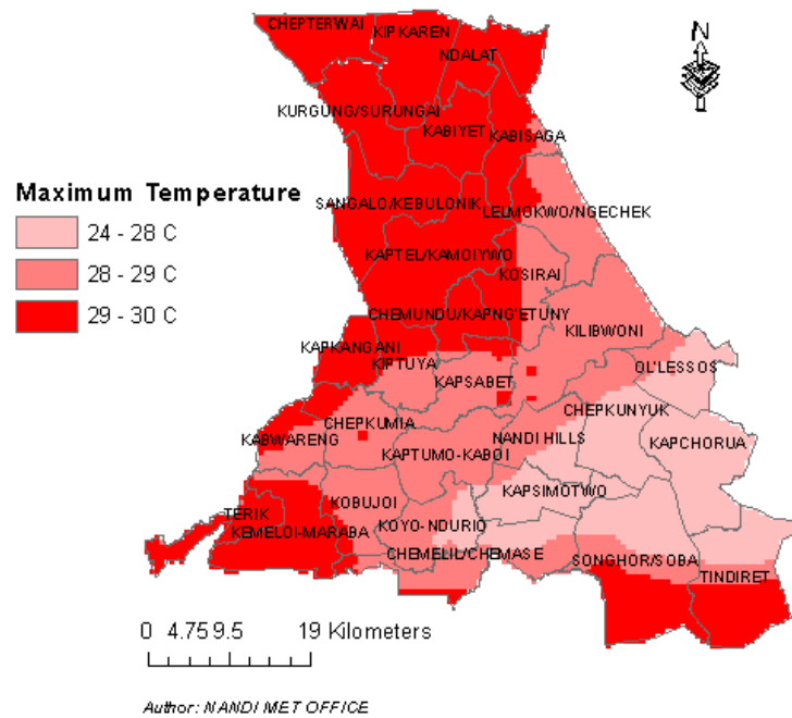
Figure 2: Average Max Temperatures for 18 th to 24 th Nov 2025
