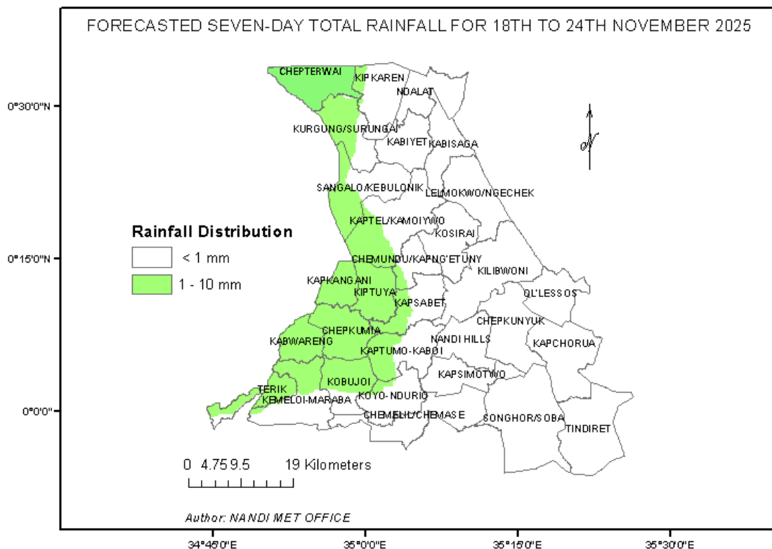
Figure 1: Forecasted Seven-Day total rainfall valid 18 th to 24 th Nov 2025
