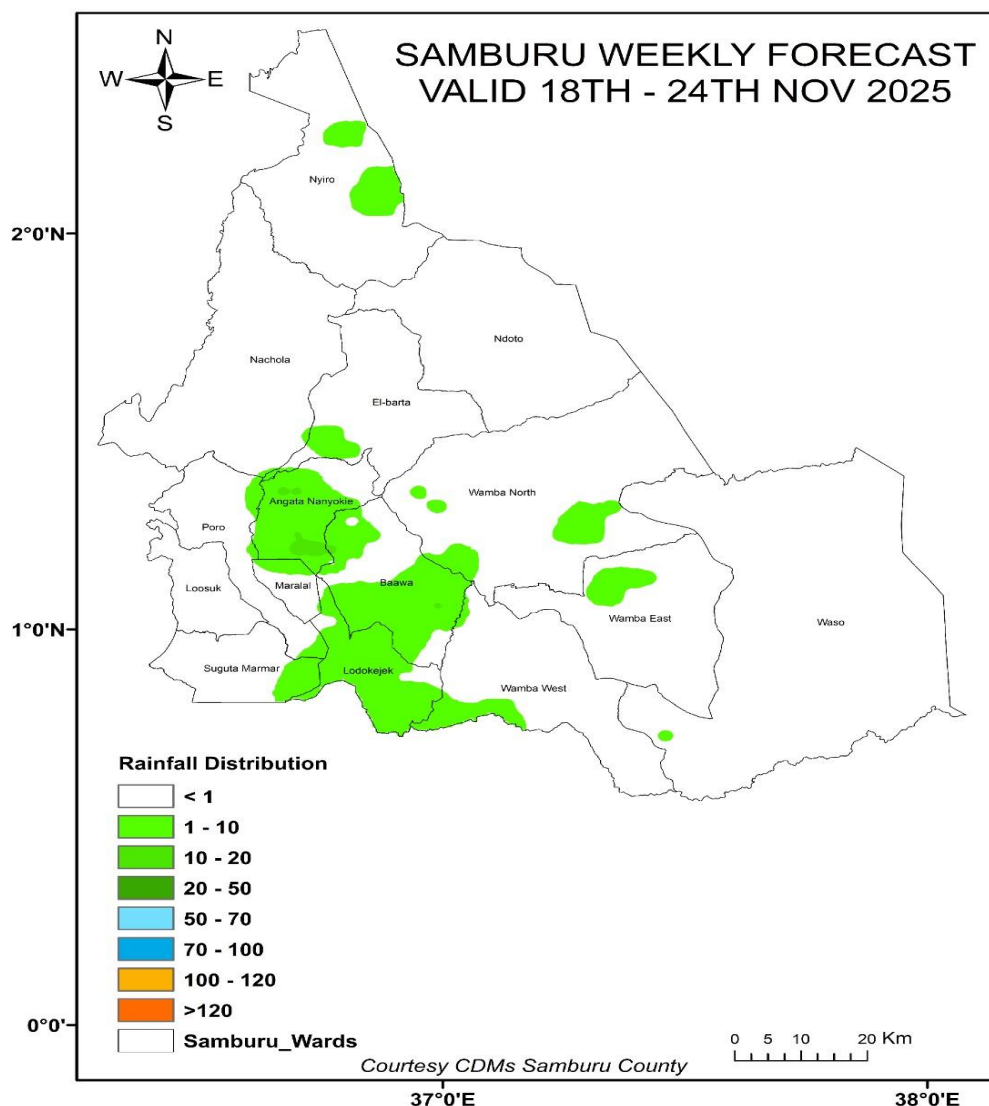
Figure 1. Samburu County Cumulative rainfall forecast
