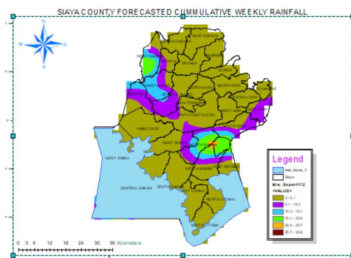
Figure 2: Forecasted cumulative weekly rainfall from 18 TH November to 24 th November 2025
