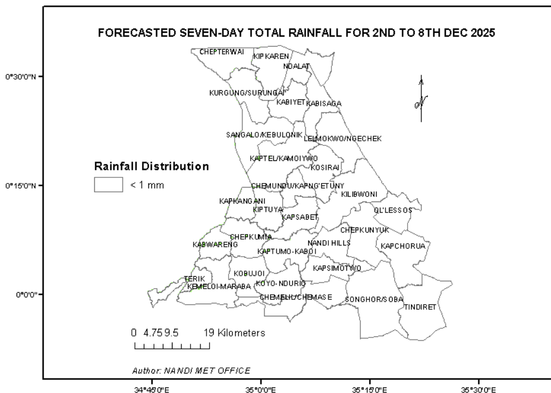
Figure 1: Forecasted Seven-Day total rainfall valid 2 nd to 8 th Dec 2025
