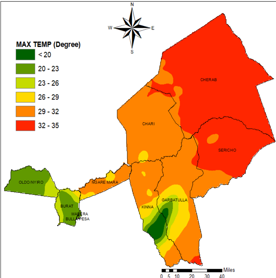
MAXIMUM TEMPERATURE FORECAST VALID 9 - 15 DEC 2025
