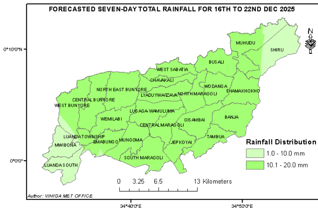
Figure 1: Forecasted Seven-Day total rainfall valid 16 th to 22 nd Dec 2025
