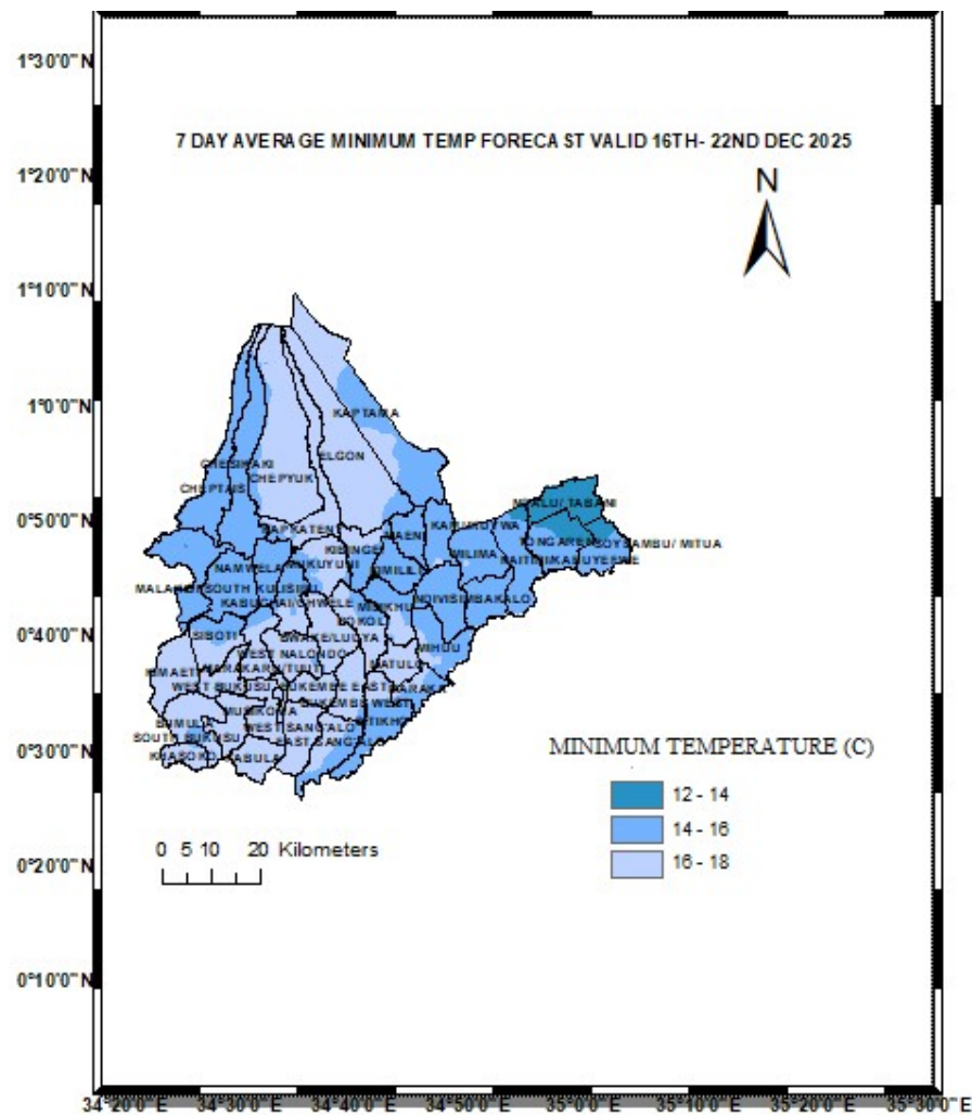
Figure 3: Expected Average Minimum Temperature valid 16 th – 22 nd December 2025
