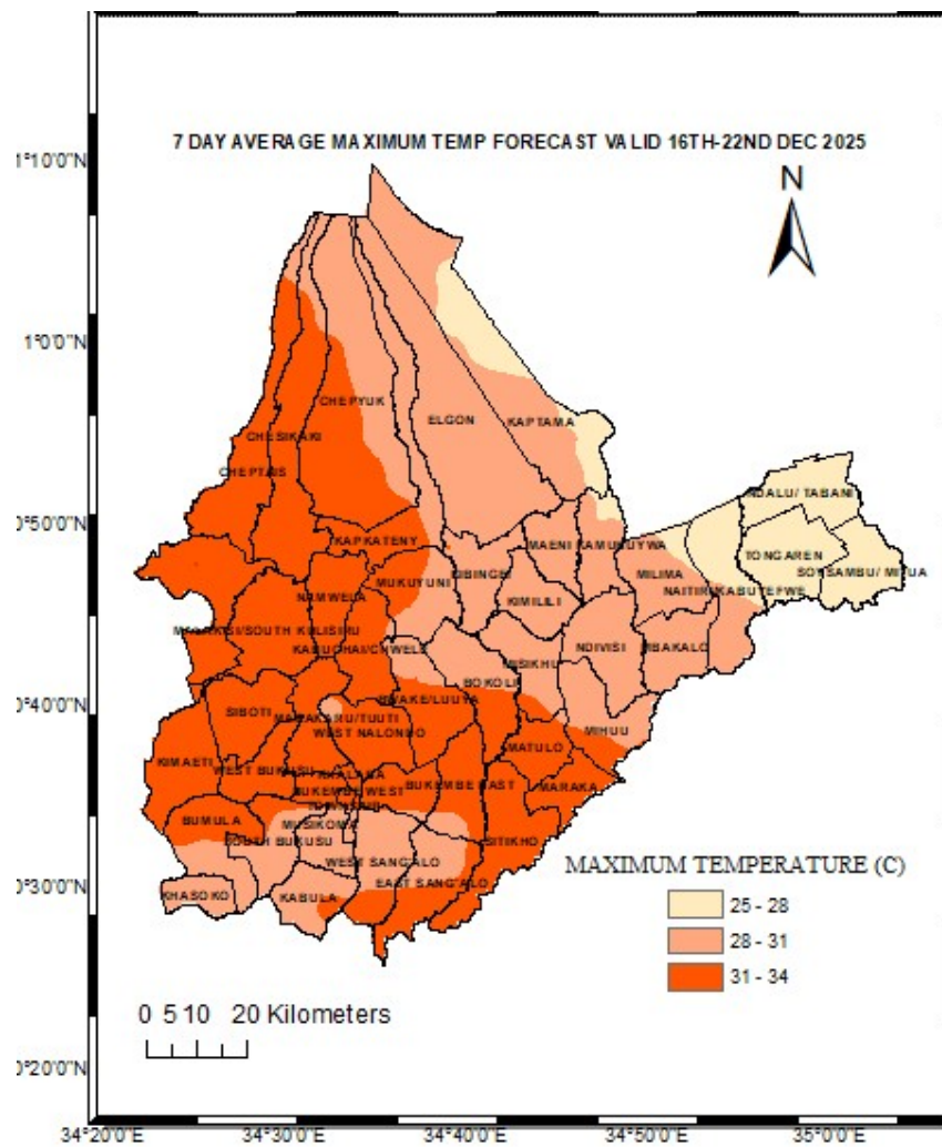
Figure 2: Expected Average Maximum Temperature valid 16 th – 22 nd December 2025
