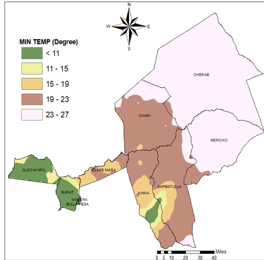
MINIMUM TEMPERATURE FORECAST VALID 16 - 22 DEC 2025
