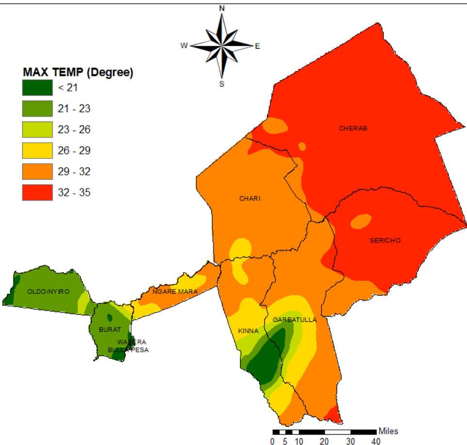
MAXIMUM TEMPERATURE FORECAST VALID 16 - 22 DEC 2025
