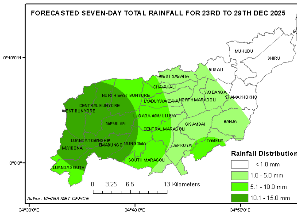
Figure 1: Forecasted Seven-Day total rainfall valid 23 rd to 29 th Dec 2025
