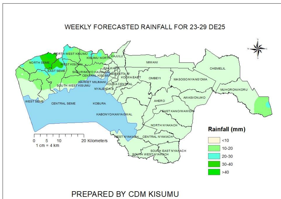
Figure 1: Cumulative rainfall forecast over Kisumu County
