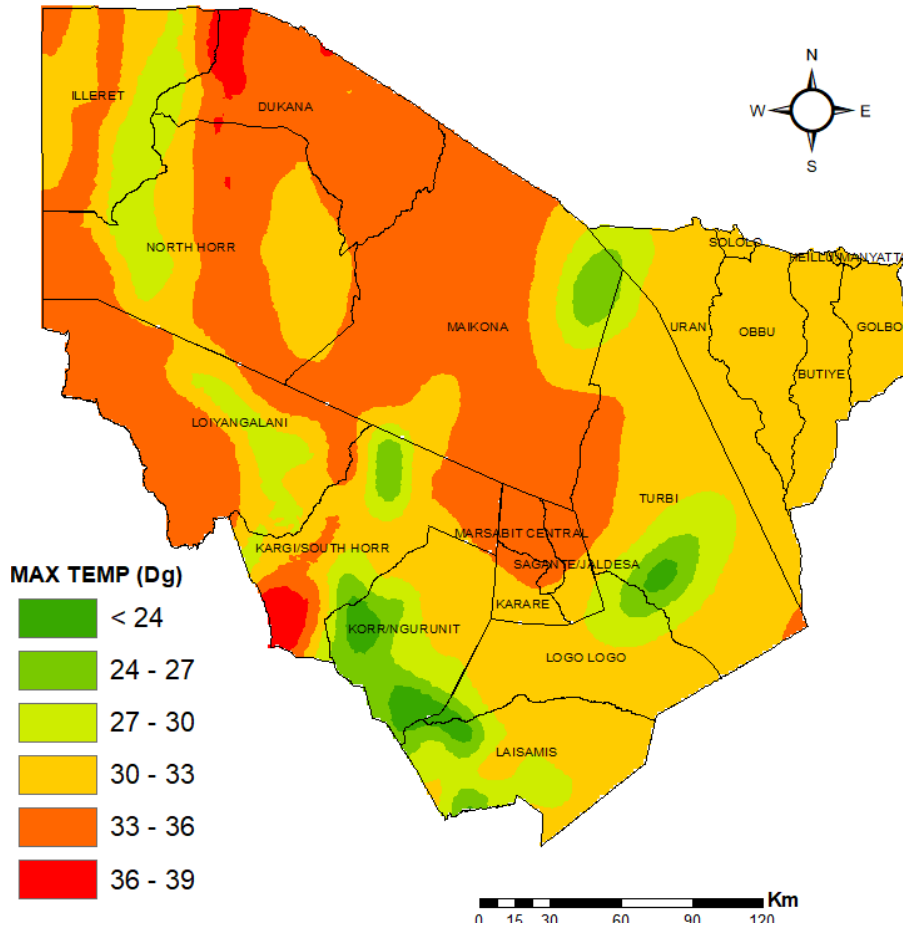
7 WEEKLY MAXIMUM TEMPERATURE FORECAST VALID 3 - 9 FEB 2026
