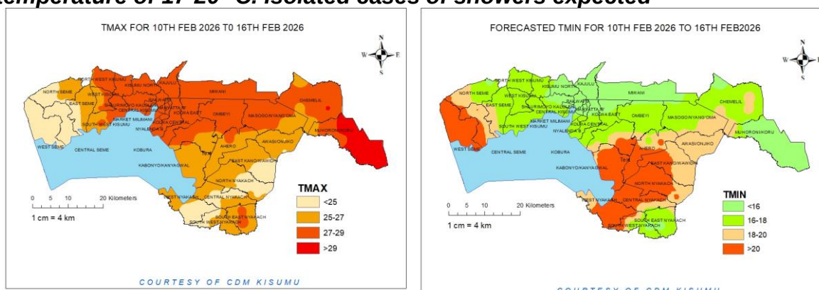
Figure 2: Average maximum (left) and minimum (right) temperature forecasts
