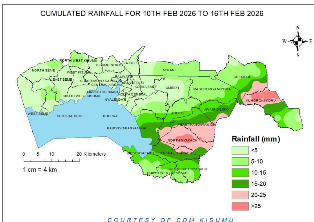
Figure 1: Cumulative rainfall forecast over Kisumu County
