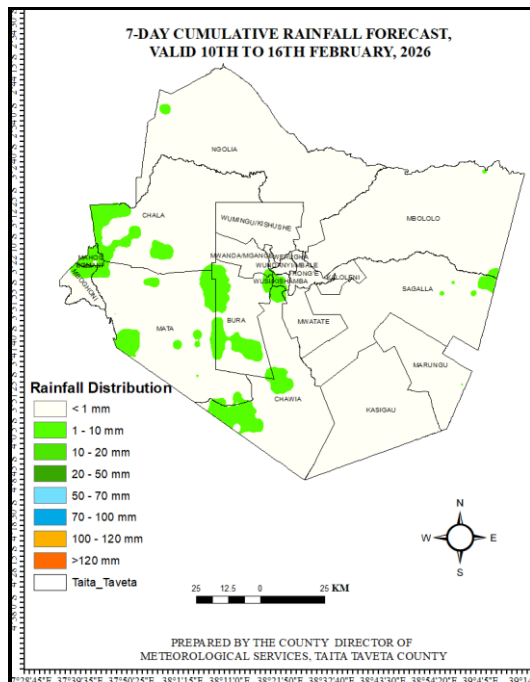
Figure 1: Expected Rainfall distribution over Taita Taveta County valid Tuesday, 10 th to Monday, 16 th February, 2026
