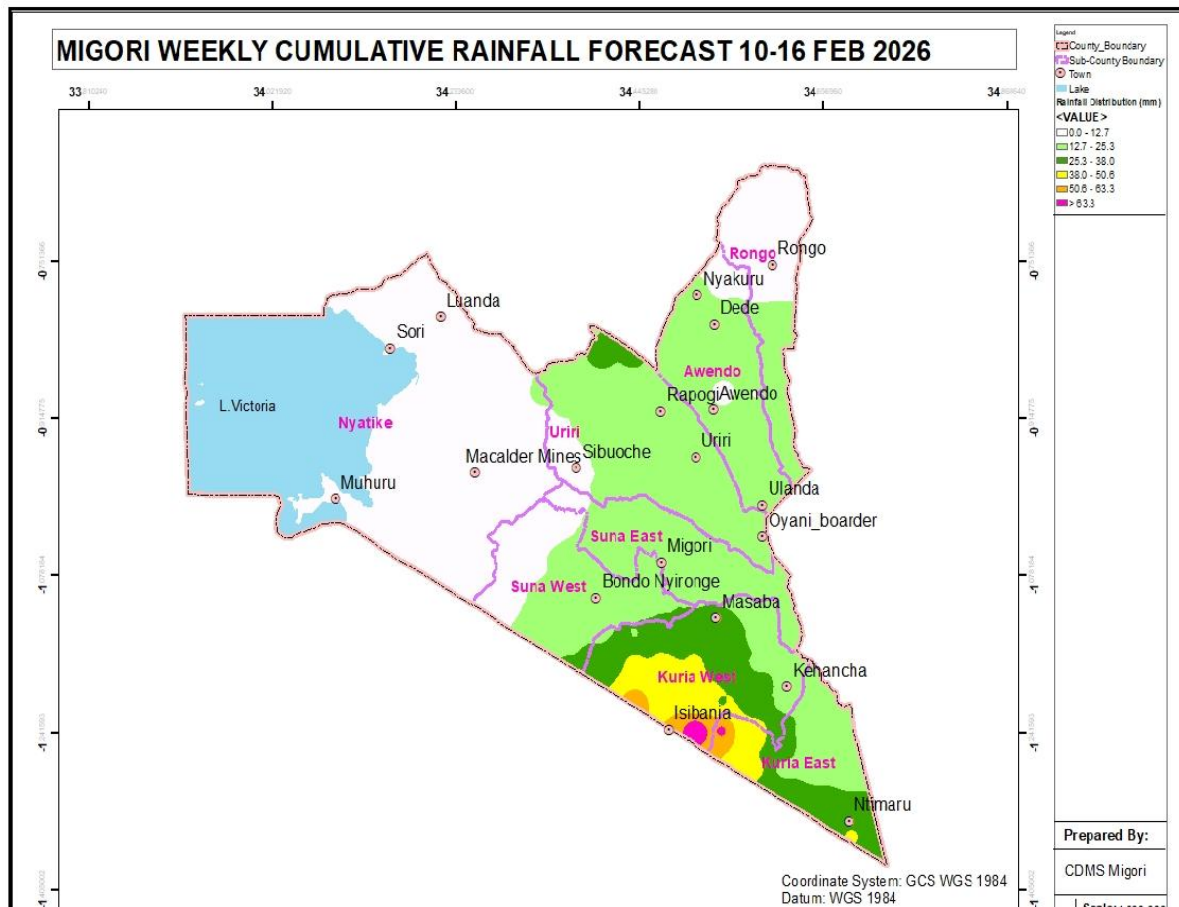
Figure 1: 7day cumulative rainfall forecast valid 10 th to 16 th February 2026
