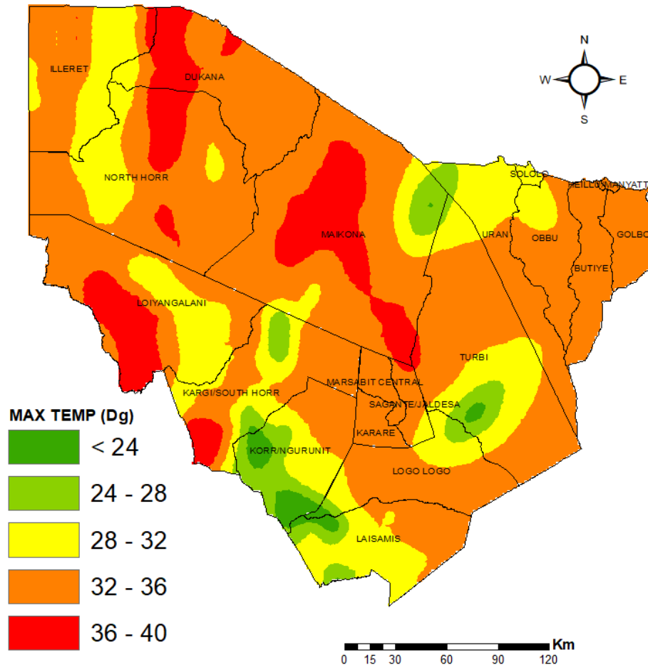
7 WEEKLY MAXIMUM TEMPERATURE FORECAST VALID 17 -- 23 FEB 2026
