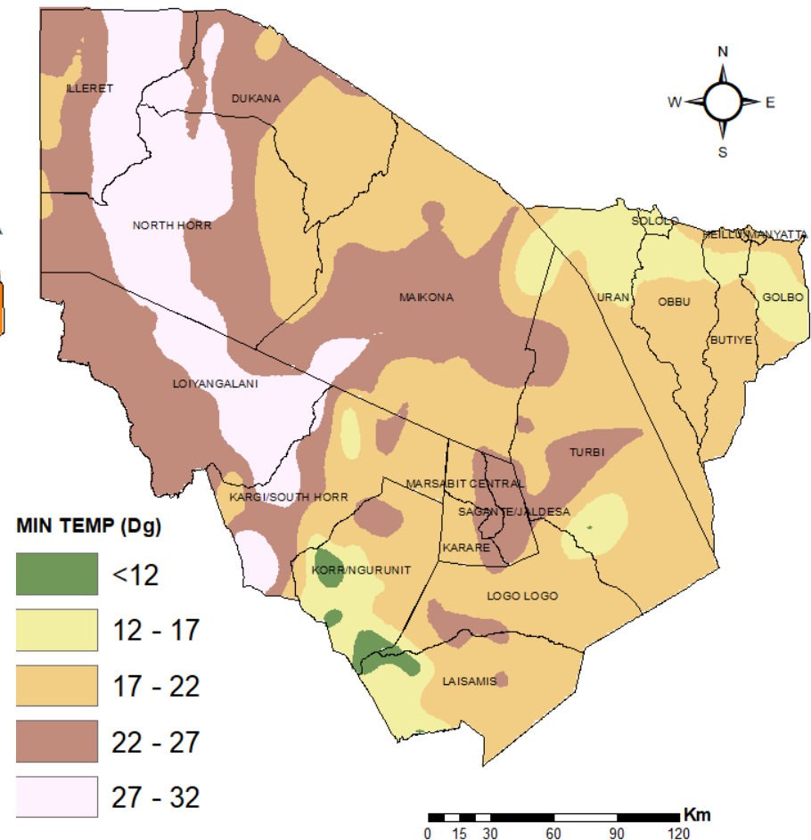
7 WEEKLY MINIMUM TEMPERATURE FORECAST VALID 17 -- 23 FEB 2026
