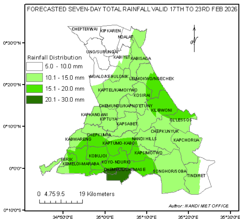
Figure 1: Forecasted Seven-Day total rainfall valid 17 th to 23 rd Feb 2026
