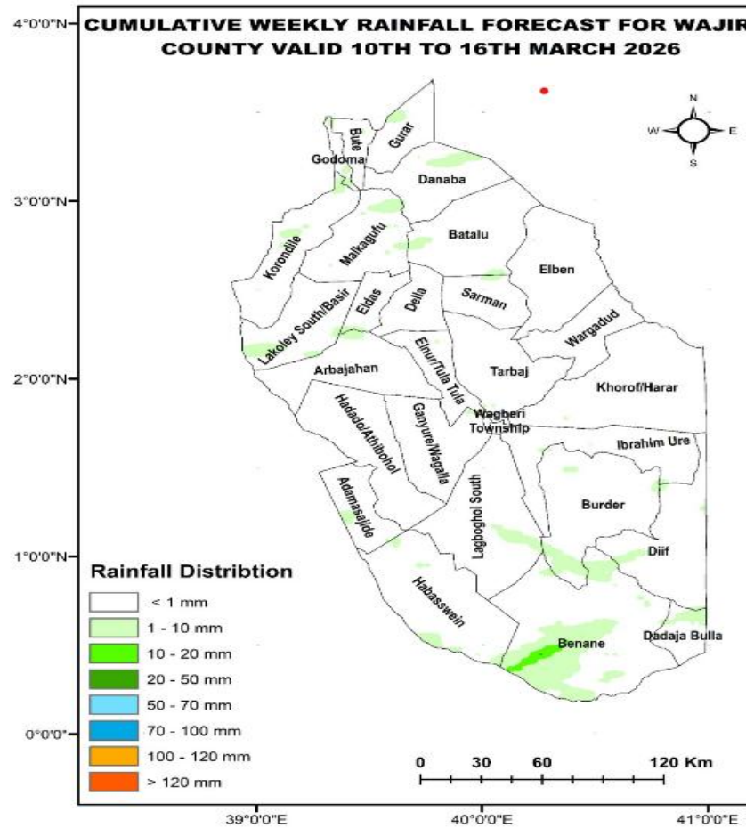
Figure1: Wajir County Weekly Cumulative Rainfall Forecast
