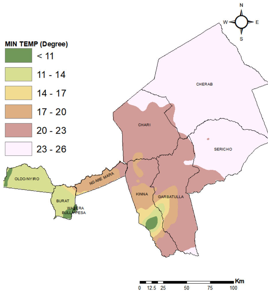
WEEKLY MINIMUM TEMPERATURE FORECAST VALID 10 - 16 MARCH 2026
