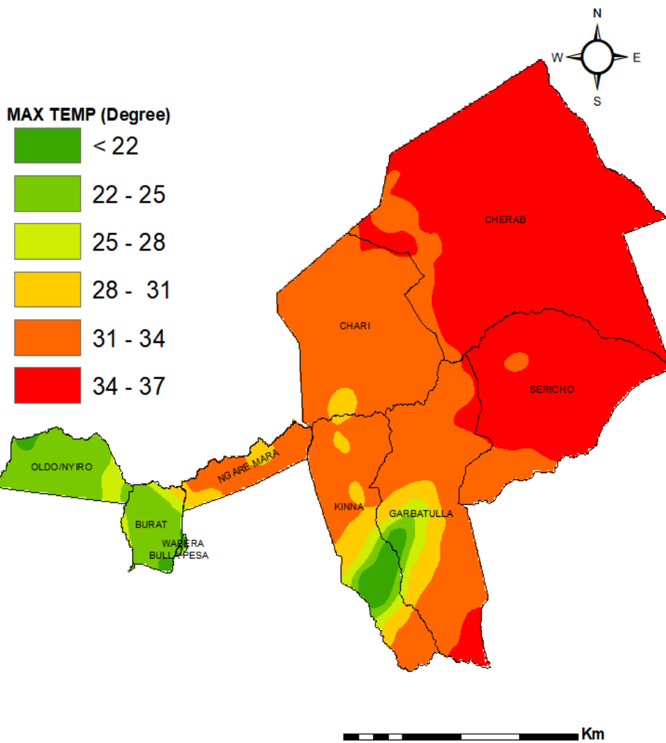
WEEKLY MAXIMUM TEMPERATURE FORECAST VALID 10 - 16 MARCH 2026
