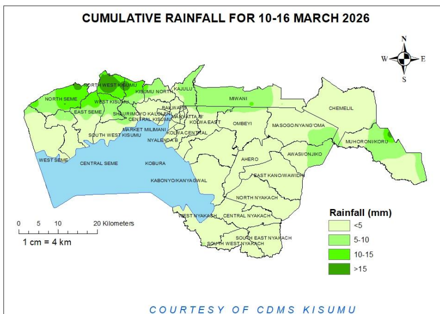
Figure 1: Cumulative rainfall forecast over Kisumu County
