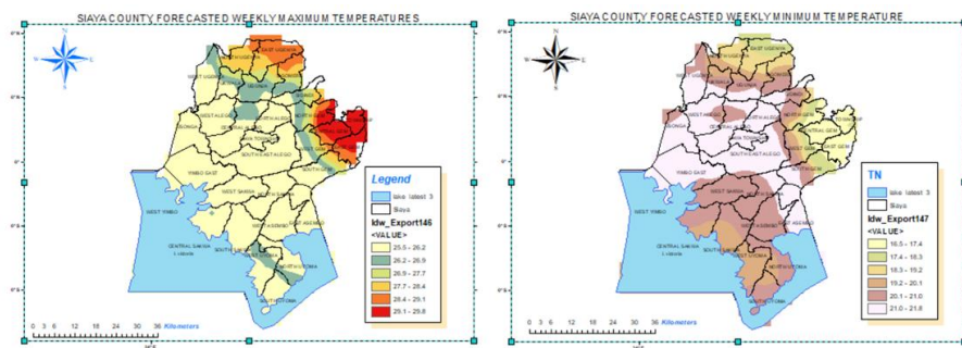
Fig: 3a Forecasted weekly maximum Temp. Fig: 3b Forecasted weekly minimum Temp.
