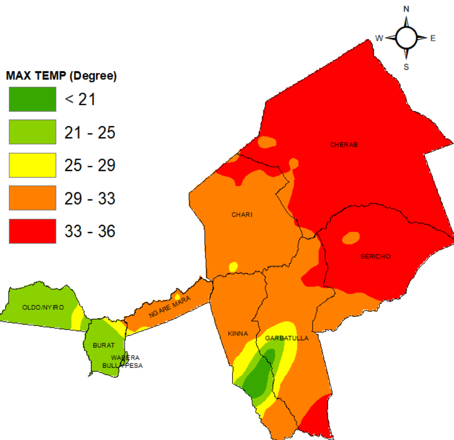
WEEKLY MAXIMUM TEMPERATURE FORECAST VALID 17 - 23 MARCH 2026
