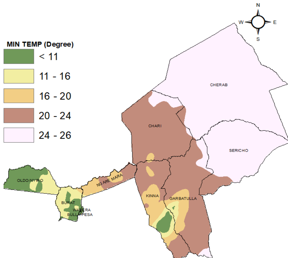
WEEKLY MINIMUM TEMPERATURE FORECAST VALID 17 - 23 MARCH 2026
