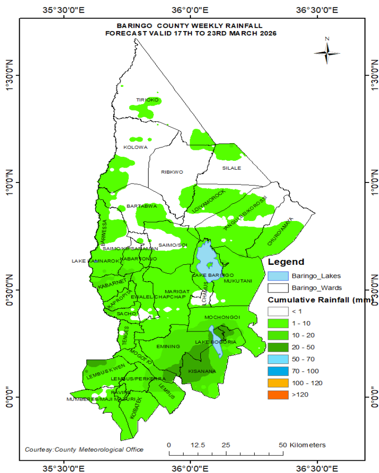
Fig 1. Forecasted cumulative rainfall amounts (mm)
