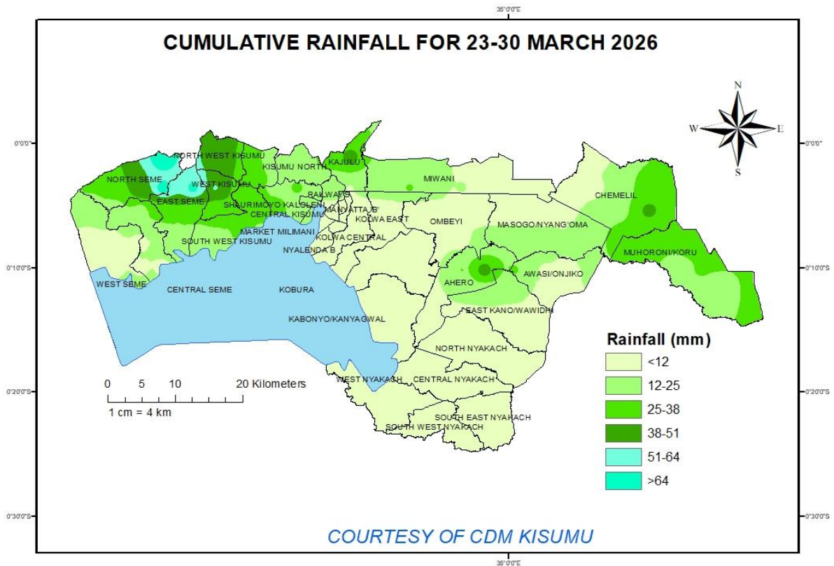
Figure 1: Cumulative rainfall forecast over Kisumu County
