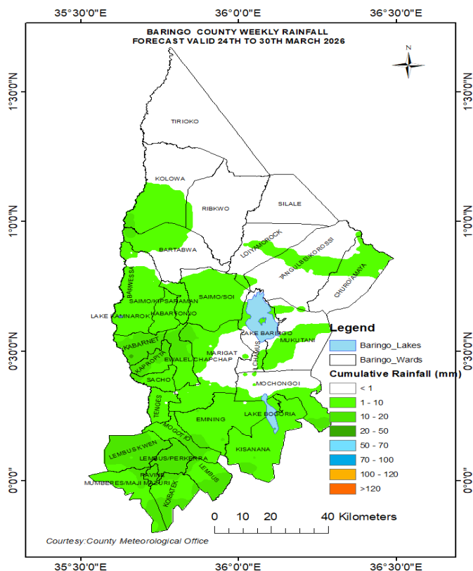
Fig 1. Forecasted cumulative rainfall amounts (mm)
