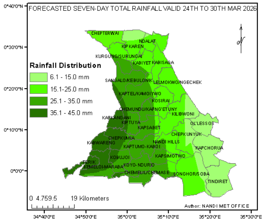
Figure 1: Forecasted Seven-Day total rainfall valid 24 th to 30 th Mar 2026
