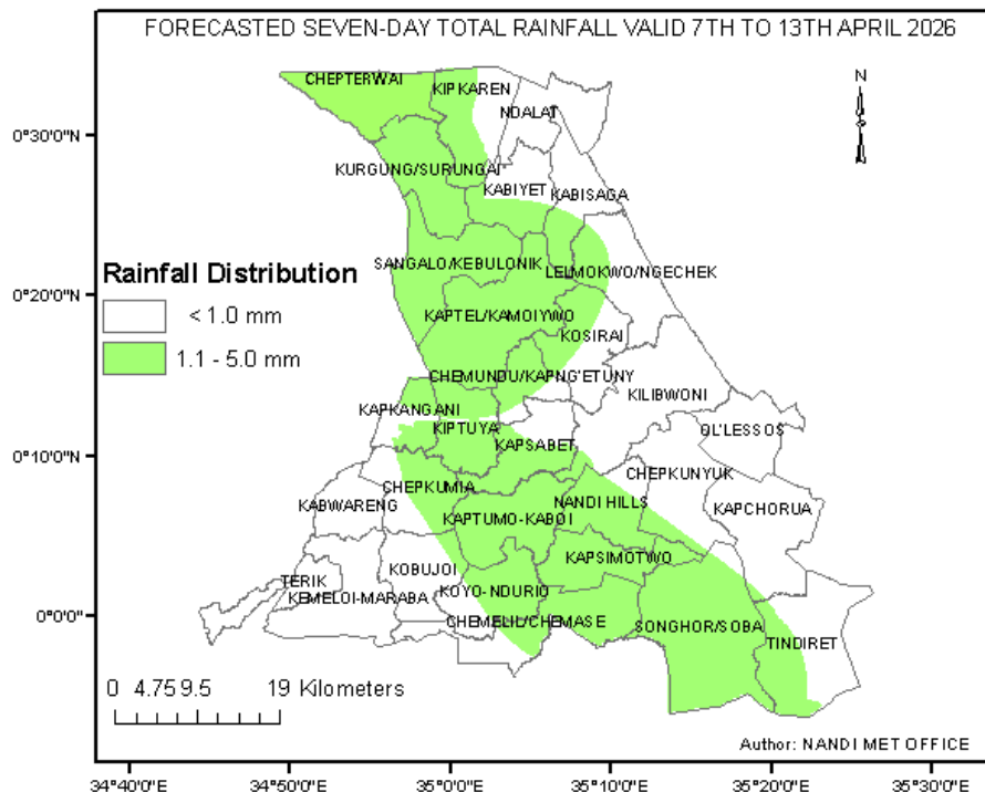
Figure 1: Forecasted Seven-Day total rainfall valid 7 th to 13 th Apr 2026
