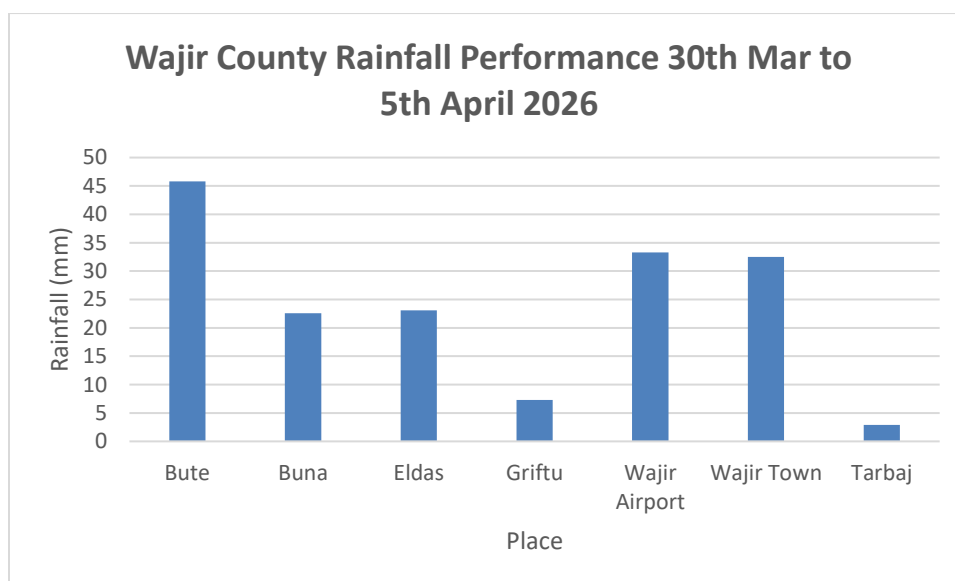
Figure 1: Rainfall Performance from 30 th Mar to 5 th April 2026
