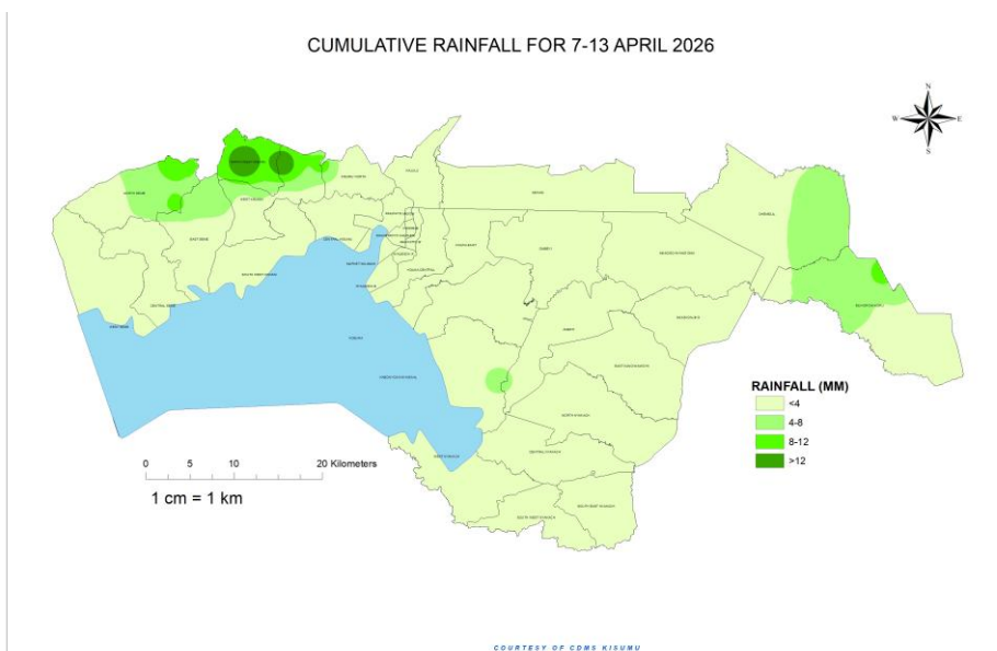
Figure 1: Cumulative rainfall forecast over Kisumu County
