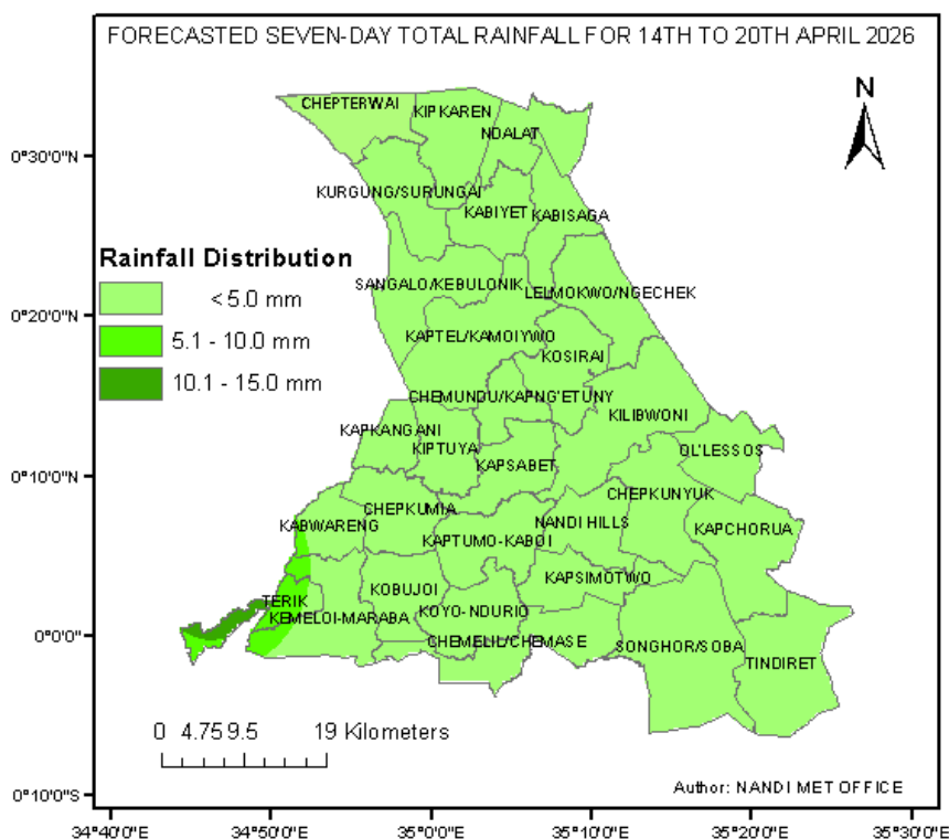
Figure 1: Forecasted Seven-Day total rainfall valid 14 th to 20 th Apr 2026
