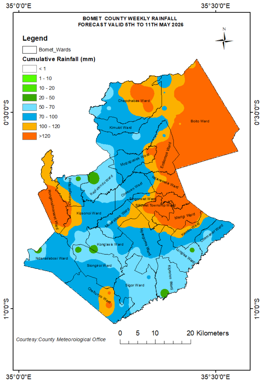
○ Fig 1. Cumulative weekly spatial rainfall distribution
