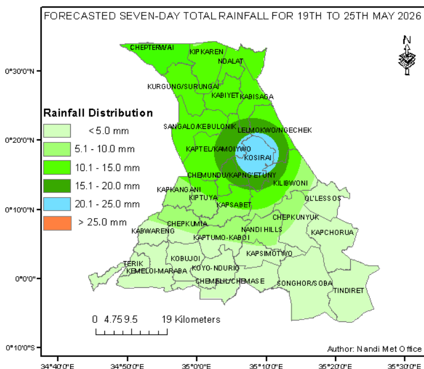
Figure 1: Forecasted Seven-Day total rainfall valid 19 th to 25 th May 2026
