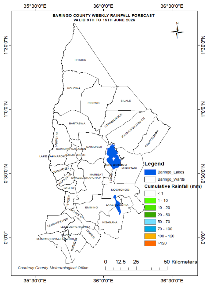
Fig 1. Forecasted cumulative rainfall amounts (mm)
