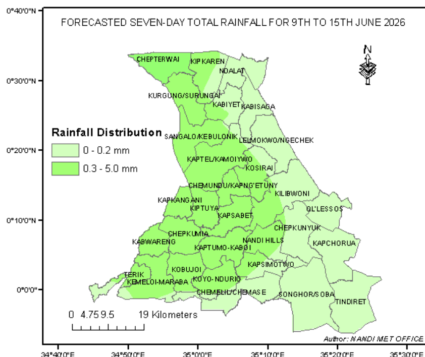
Figure 1: Forecasted Seven-Day total rainfall valid 9 th to 15 th Jun 2026
