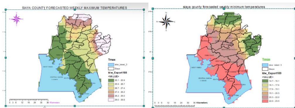
Figure 3a: Forecasted weekly Maximum temperatures
