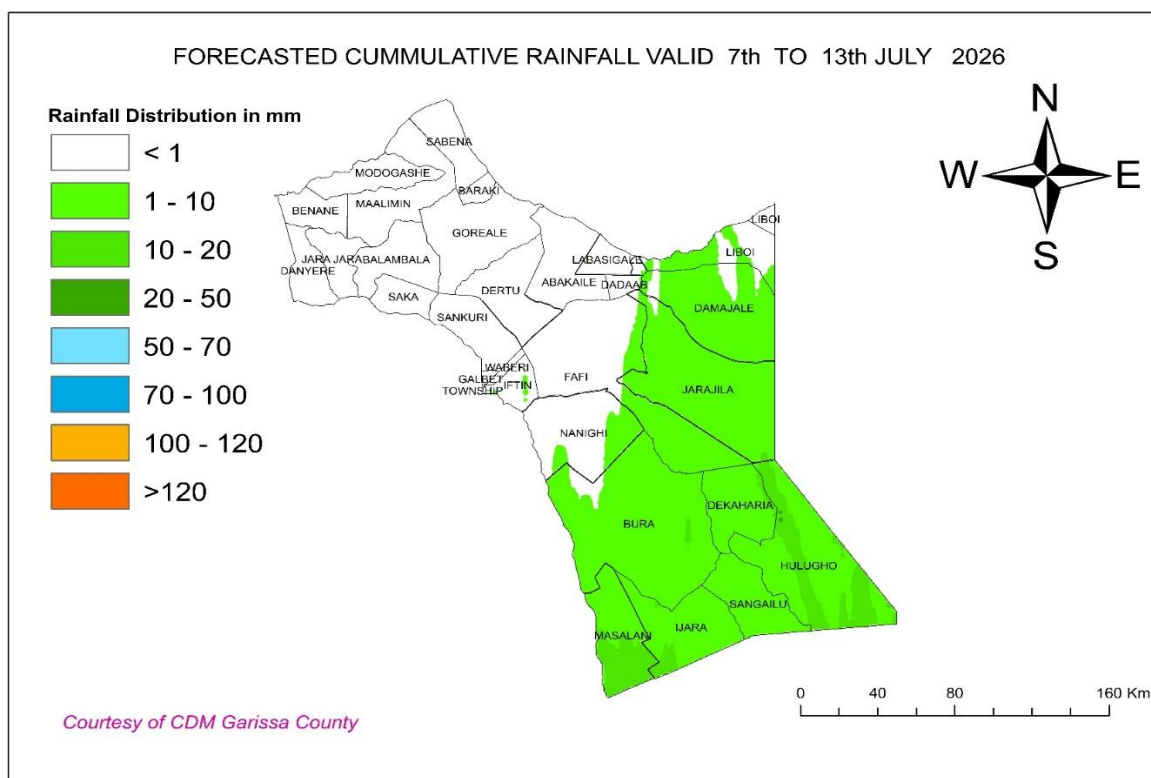
Figure 1: Expected Rainfall distribution over Garissa County valid Tuesday 07 th to Monday 13 th July 2026
