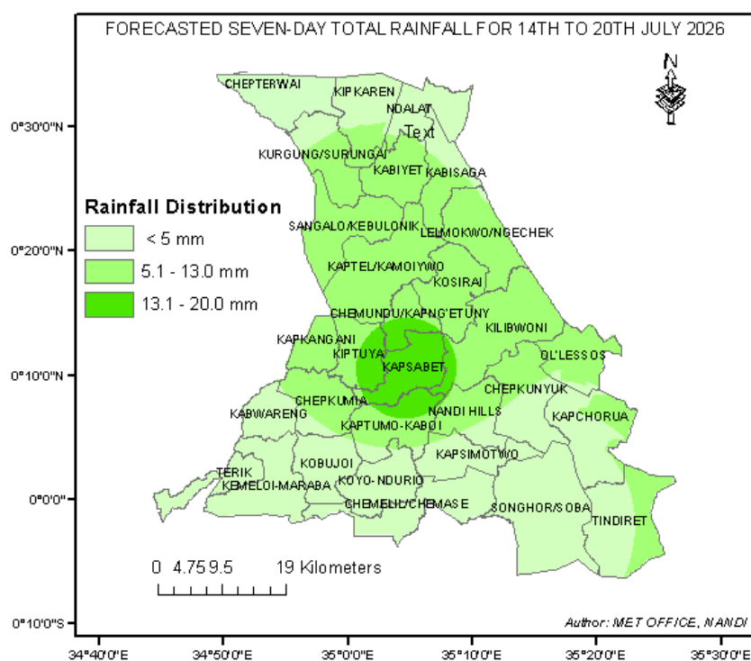
Figure 1: Forecasted Seven-Day total rainfall valid 14 th to 20 th July 2026
