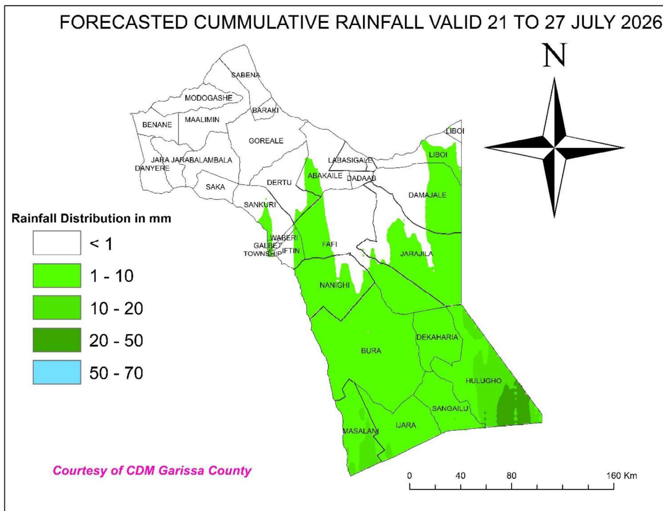
Figure 1: Expected Rainfall distribution over Garissa County valid Tuesday 21 ST to Monday 27 th July 2026
