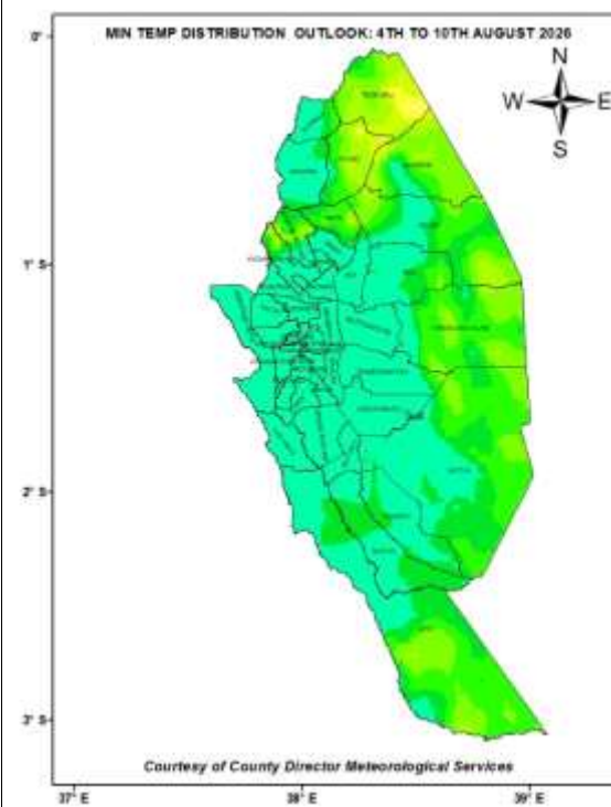
Figure 3: Forecasted Seven-Day Mean Mini Temperatures for 4 th to 10 th August 2026
