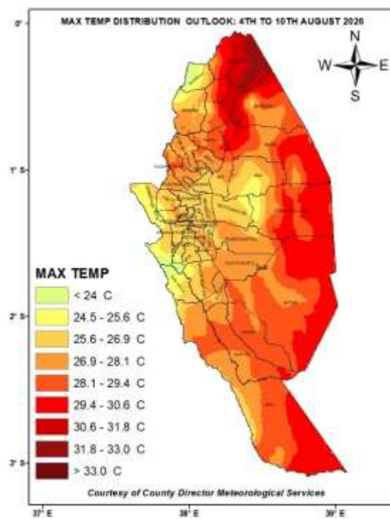
Figure 2: Forecasted Seven-Day Mean Max Temperatures for 4 th to 10 th August 2026
