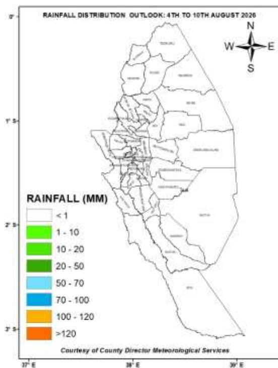
Figure 1: Forecasted Seven-Day Total Rainfall for 4 th to 10 th August 2026
