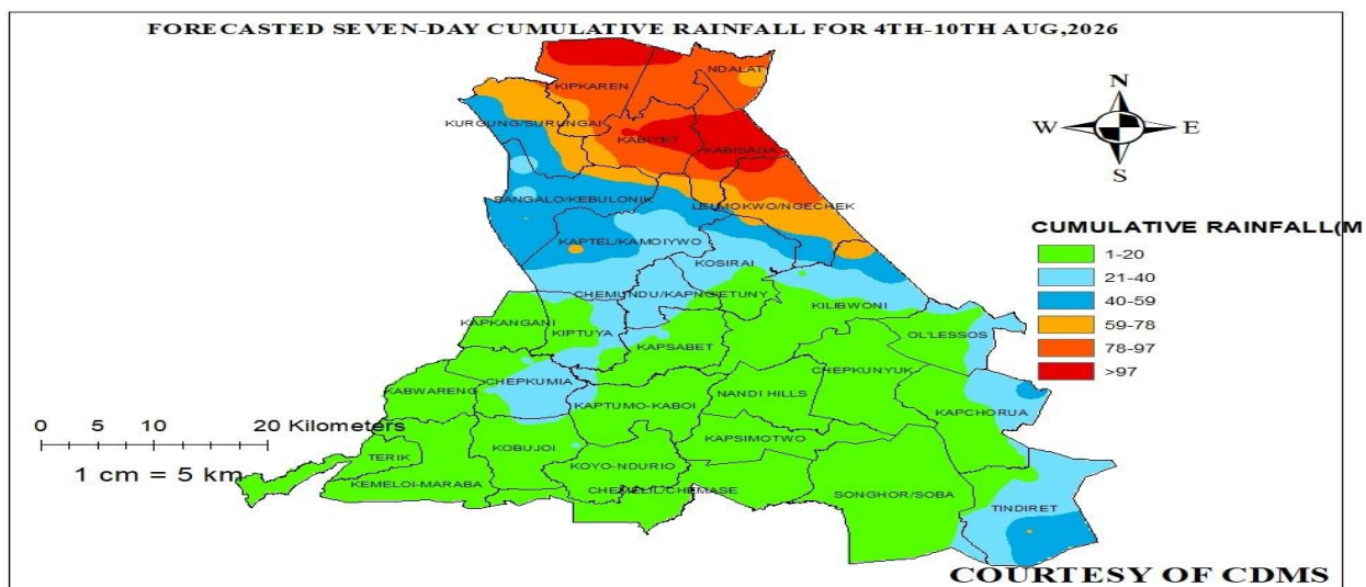
Figure 1: Forecasted Seven-Day total rainfall valid 4 TH -10 TH Aug 2026
